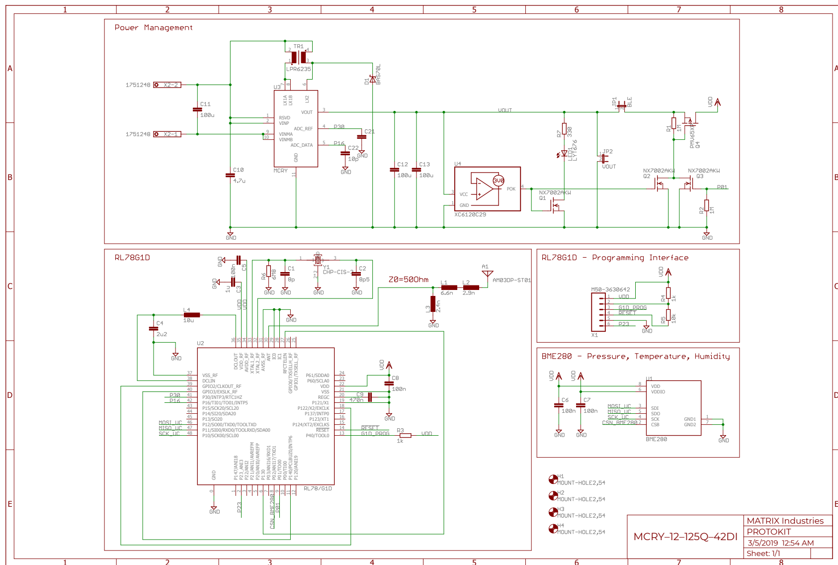
Figure 6: MCRY-PROTOKIT Schematics
